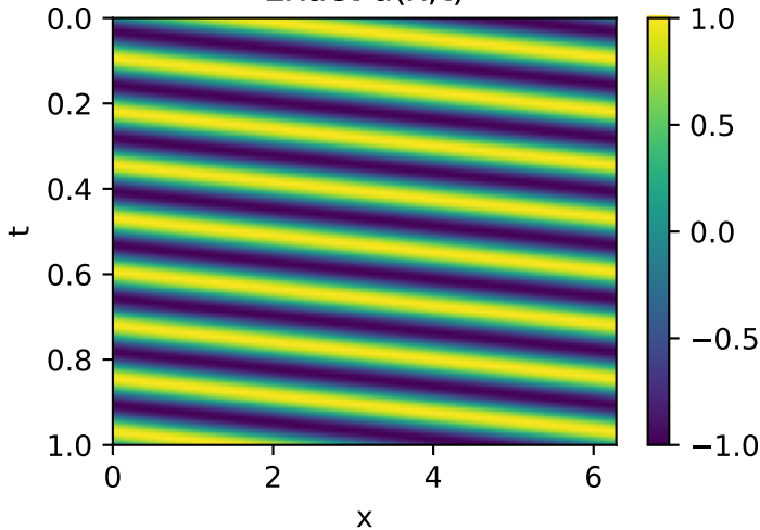
Exact u(x,t)
